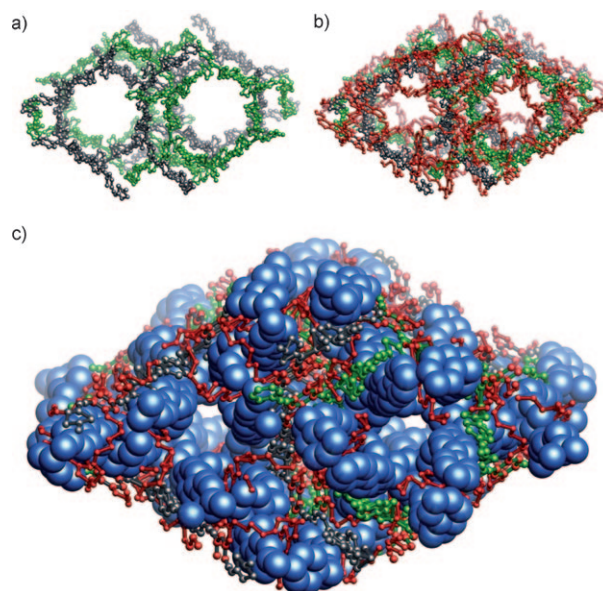
Figure 6. Catenated struts in catenated MOF-1030. a) View of MOF-1030 along the c axis. Crown ethers and \text{CBPQT}^{4+} rings are omitted. MOF-1030 is a catenated structure with two different frameworks shown in two different colors (gray and green). b) The framework with crown ethers represented in red. Hydrogen atoms, anions, and \text{CBPQT}^{4+} rings are omitted. c) Two interwoven nets, one in gray and the other in green, with the crown ethers shown in red and the \text{CBPQT}^{4+} rings in blue and featured in a space-filling manner.
